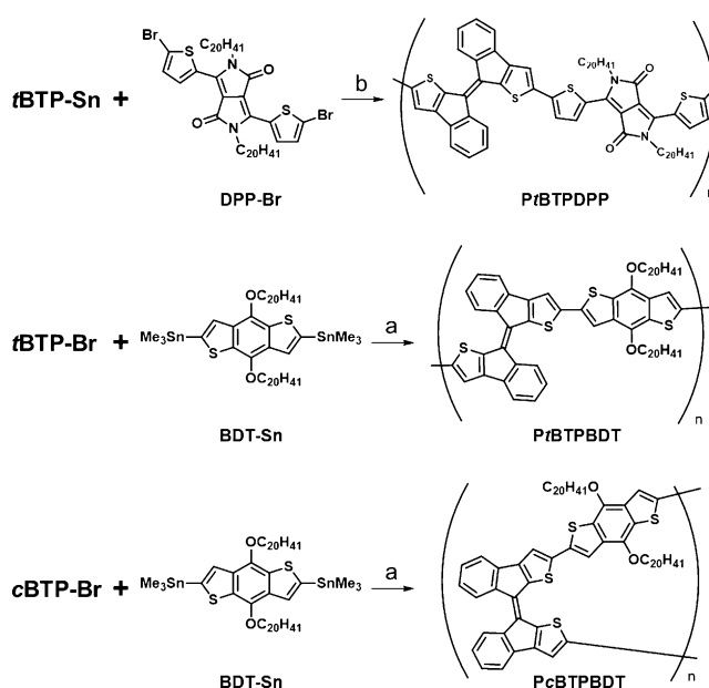
Scheme 3. Synthesis of BTP-based conjugated polymers by Stille coupling. a) [\text{Pd}_2(\text{dba})_3] , P( o -tol), chlorobenzene; b) [\text{Pd}_2(\text{dba})_3] , P( o -tol), chlorobenzene, microwave reaction.
