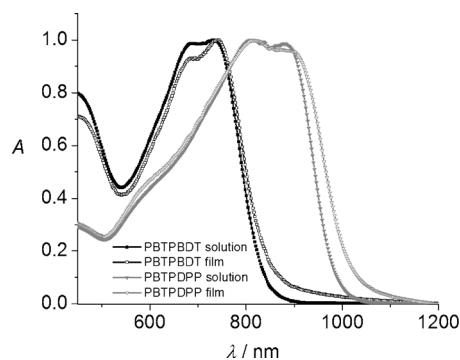
Figure 5. UV/Vis absorption of trans -PBTPBDT and trans -PBTPDPP in solutions and as-cast films.
