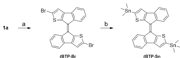
Scheme 2. Synthesis of brominated trans -BTP ( tBTP-Br ) and stannylated trans -BTP ( tBTP-Sn ). a) NBS, DCM; b) n BuLi, hexane and then \text{SnMe}_3\text{Cl} , THF.
